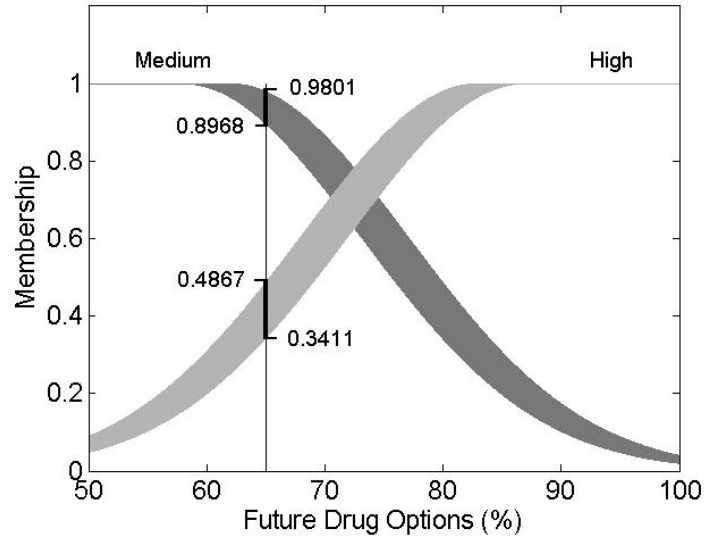
Figure 2.7: Determining the fuzzy event transition matrix for regimen 2
