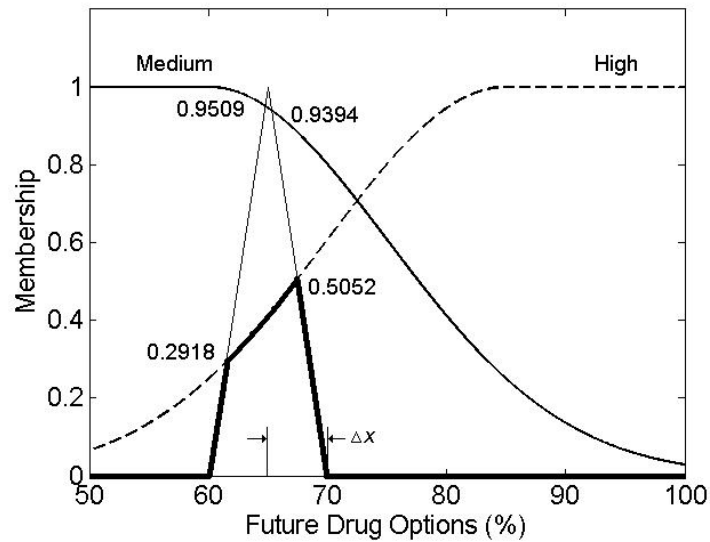
Figure 2.5: Determining the fuzzy event transition matrix for regimen 2 under the scenario 2
