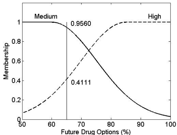
Figure 1.2: Two type-1 fuzzy sets defined for future drug options in the FDES system. In case of regimen 2, after fuzzification of the 65%, 0.9560 and 0.4111 are obtained as memberships for “Medium” and “High”.
