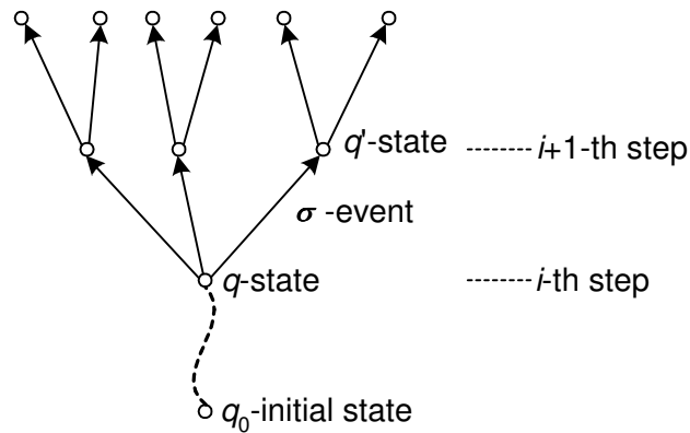
Figure 1.3: For FDES, q and q' in an example forward-looking tree for optimal control synthesis are fuzzy states represented by a vector containing the fuzzy state vectors.
