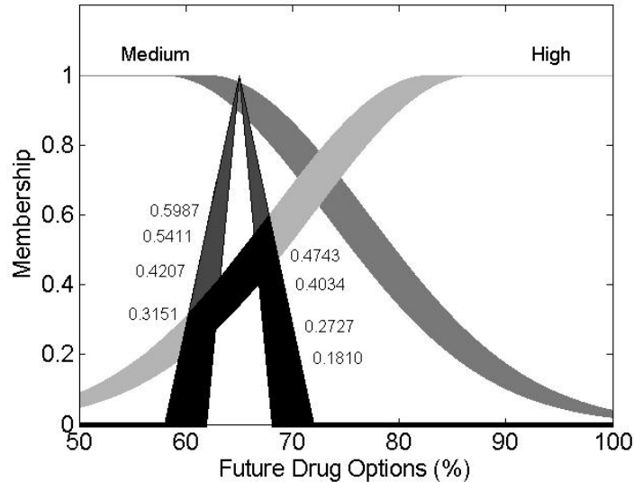
Figure 2.10: Determining the fuzzy event transition matrix for regimen 2 under the scenario 7
