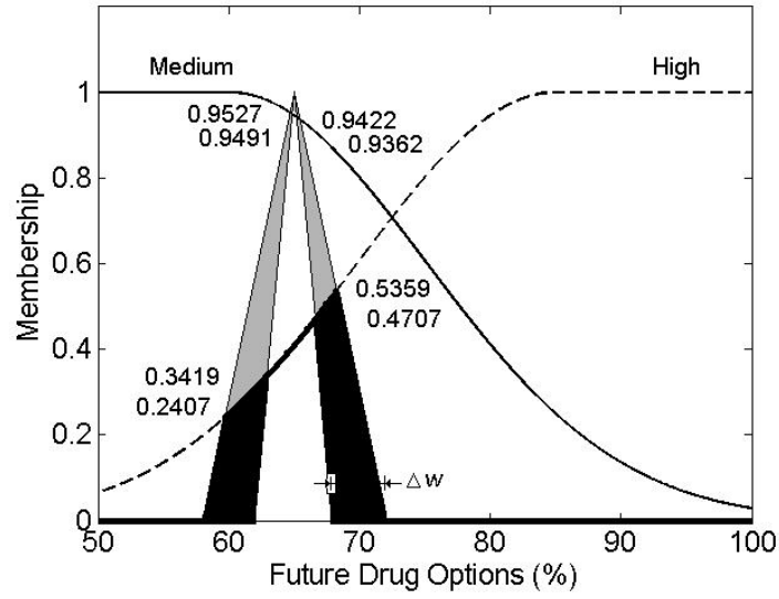
Figure 2.6: Determining the fuzzy event transition matrix for regimen 2 under the scenario 3
