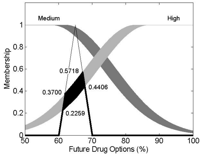
Figure 2.9: Determining the fuzzy event transition matrix for regimen 2 under the scenario 6
