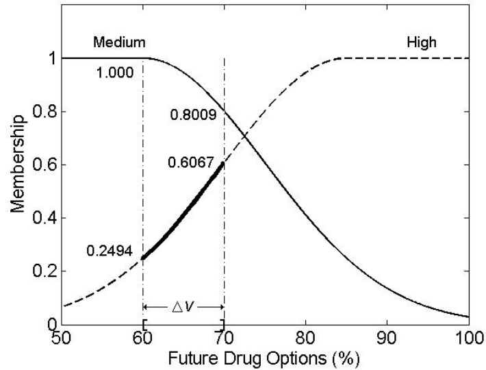
Figure 2.4: Determining the fuzzy event transition matrix for regimen 2 under the scenario 1
