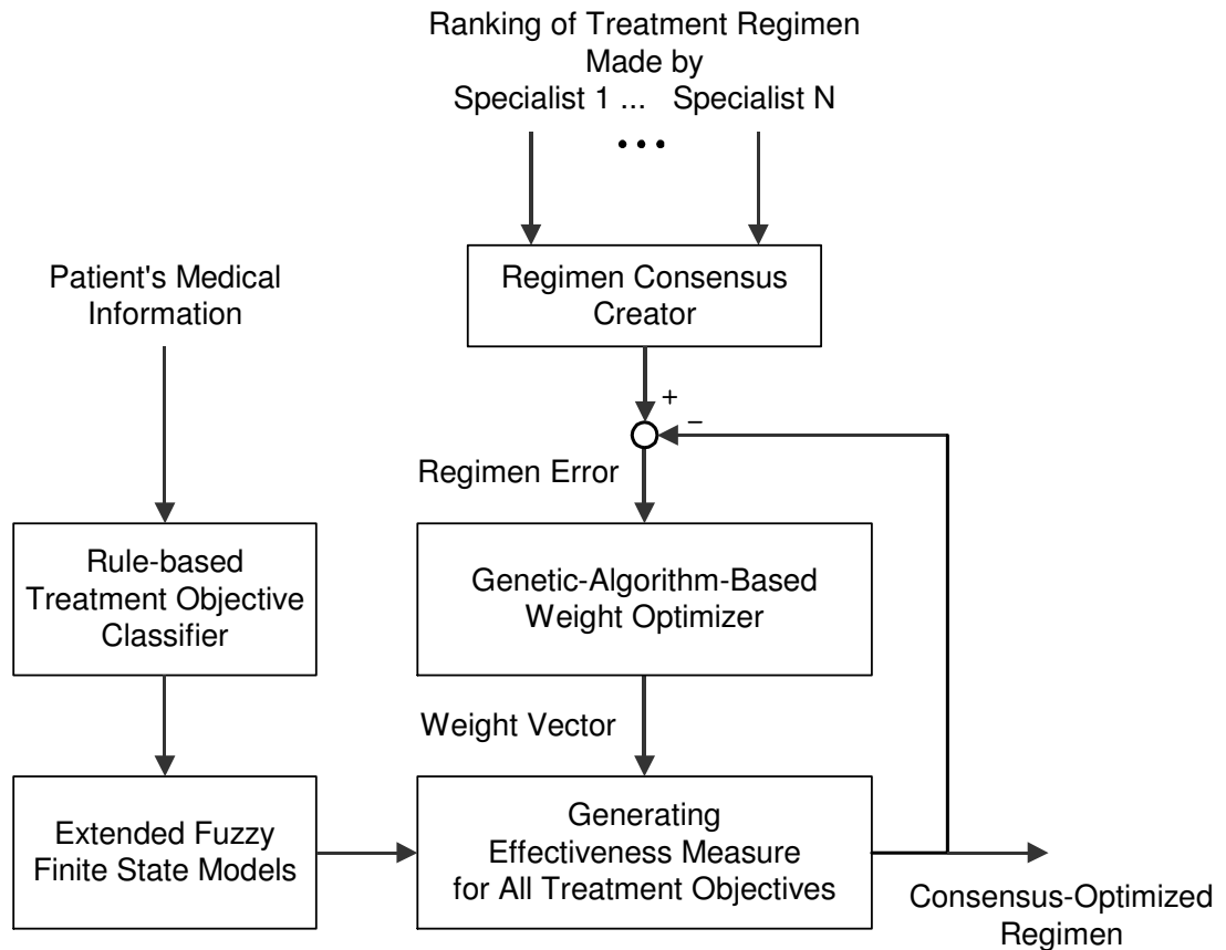
Figure 3.1: Block diagram of the EFDES-based HIV/AIDS treatment selection system with self-learning
