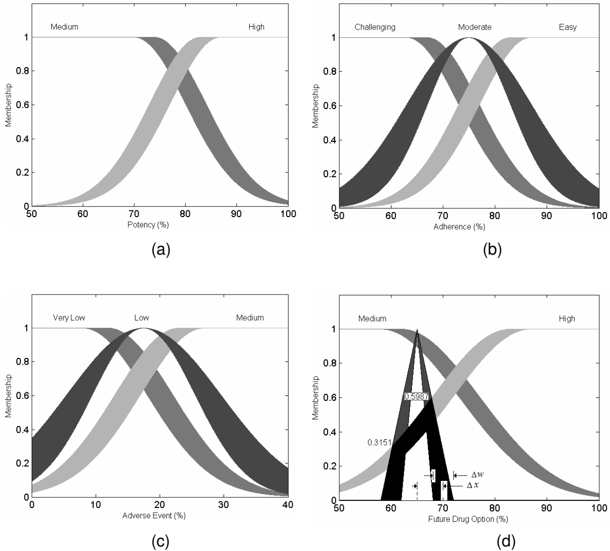
Figure 2.2: Graphical representations of the FOU of the corresponding type-2 fuzzy sets with \Delta m being 2% according to Table 2.6. Also, an example demonstration of the fuzzification process shown in (d) in which the black area of FOU fuzzified from the “High” future drug options and the characteristic of future drug options for a particular regimen represented by the interval type-2 fuzzy set and its FOU shown as a shade of the triangular shape with \Delta x being 5% and \Delta w being 4%.
