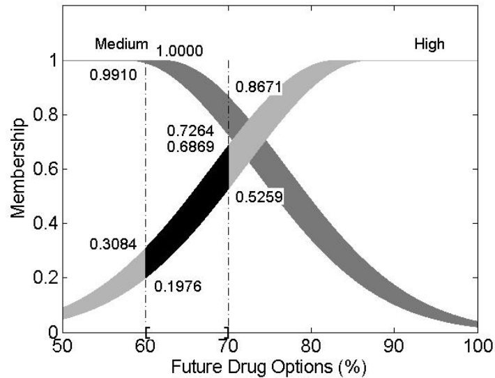
Figure 2.8: Determining the fuzzy event transition matrix for regimen 2 under the scenario 5
